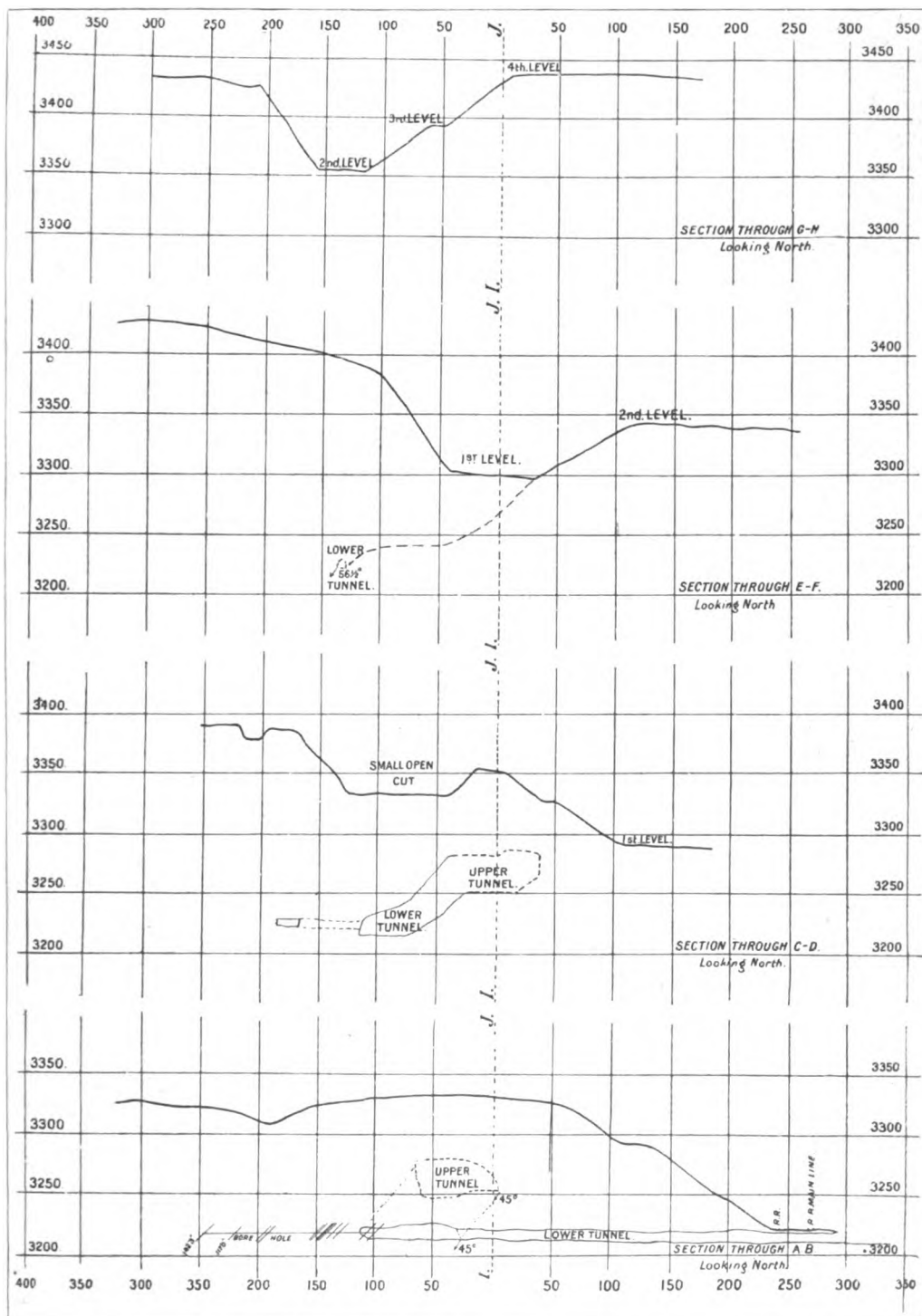
CRANBERRY MINE, VERTICAL SECTIONS THROUGH G-H, E-F, C-D, AND A-B OF PLATE XIX.
