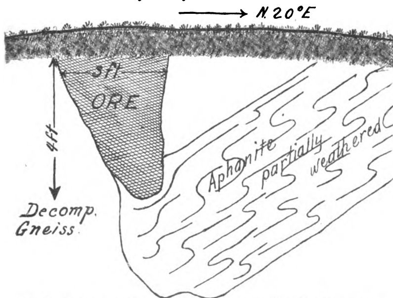
Fig. 44.—Showing relation of ore body and trap-dike, Joel Gouge place.
