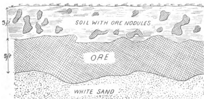
Fig. 3.—Showing section of ore bed at the Bloomery mine, Nash county.
